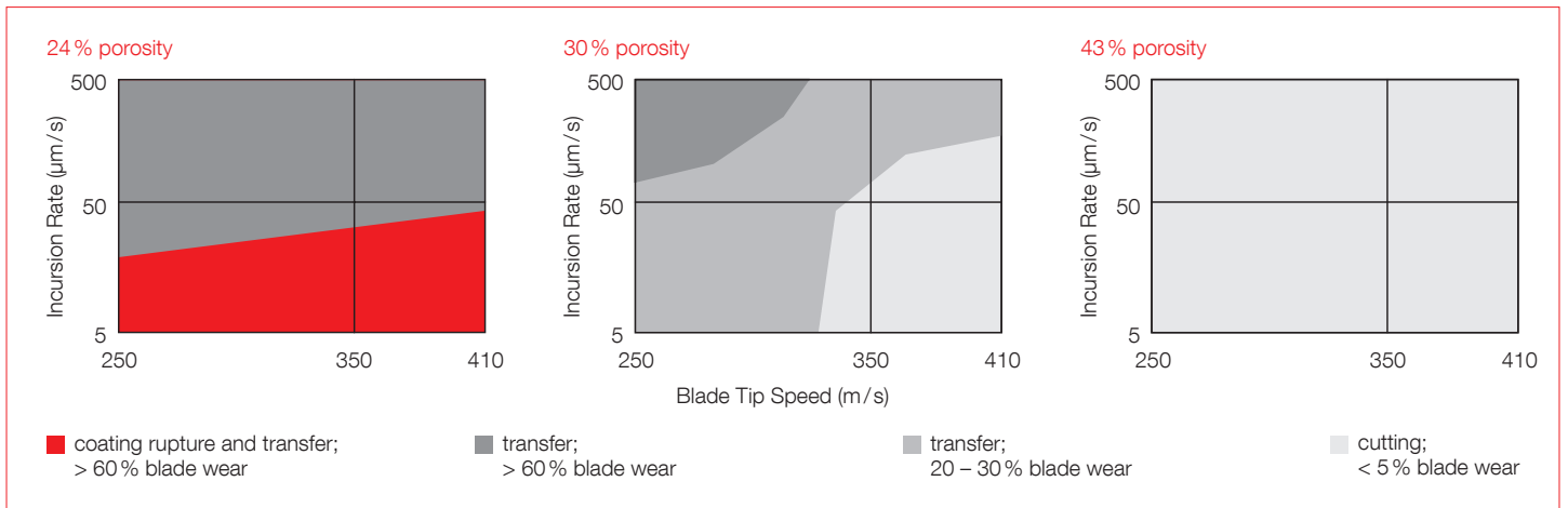
Sample abrasible wear map results at varying levels of porosity against untipped blades
