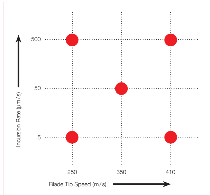
Standard 5-Point Wear Map Typical total incursion = 0.7 mm (0.028 in) Standard blade material IN 718 (bare/tipped)
