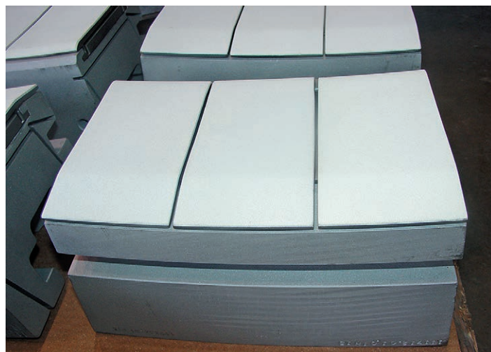
Oerlikon Metco's ceramic abrasible solutions, applied to 1 st stage HPT shroud segments, are proven to increase overall efficiency by > 1 %.
