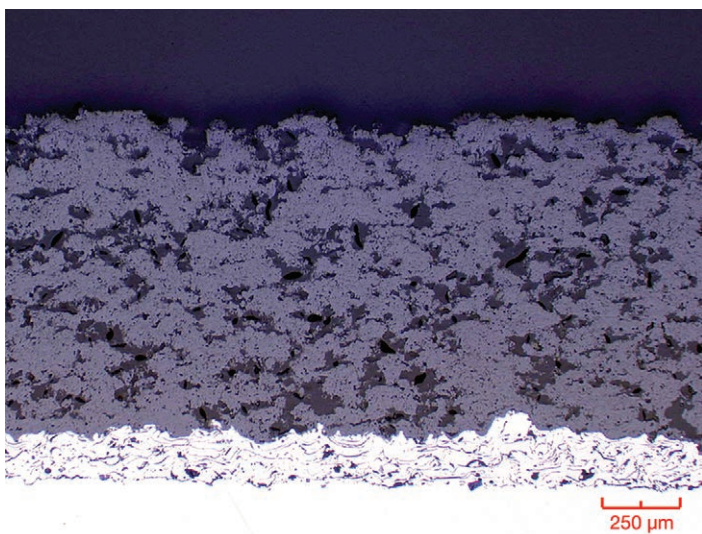
Typical microstructure of a high temperature ceramic abrasible, shown over an MCrAlY bond coat material.
