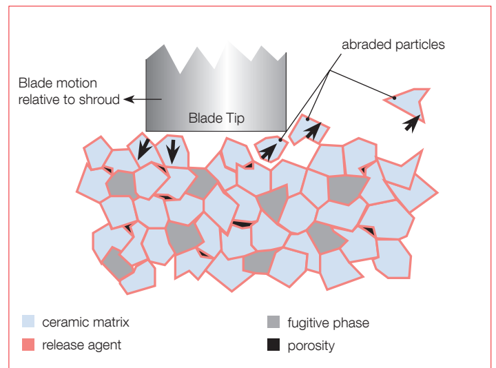
Schematic representation of the abrasible mechanism in service.
