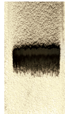
Heavy blade material transfer
