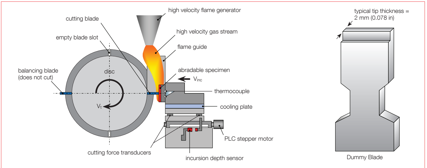
High Temperature Abradability Test Rig
