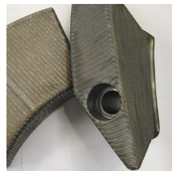
Kneader teeth with PlasmaDur 51302 wear-resistant tungsten-carbide coating
